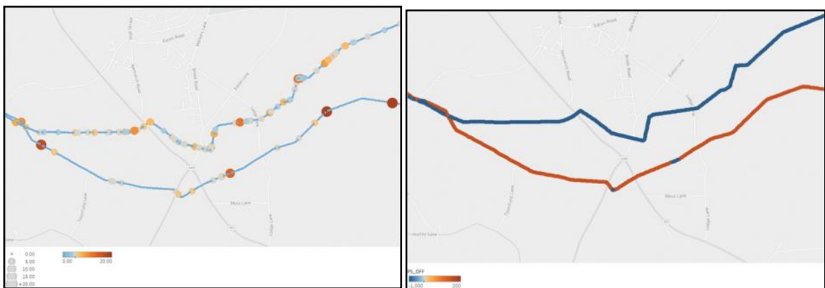
Examples of Metal Loss and CIPS Survey Results Mapped onto Pipes
