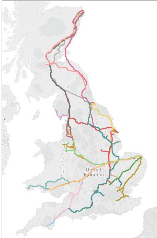
Individual Pipelines within the Gas Transmission Network
