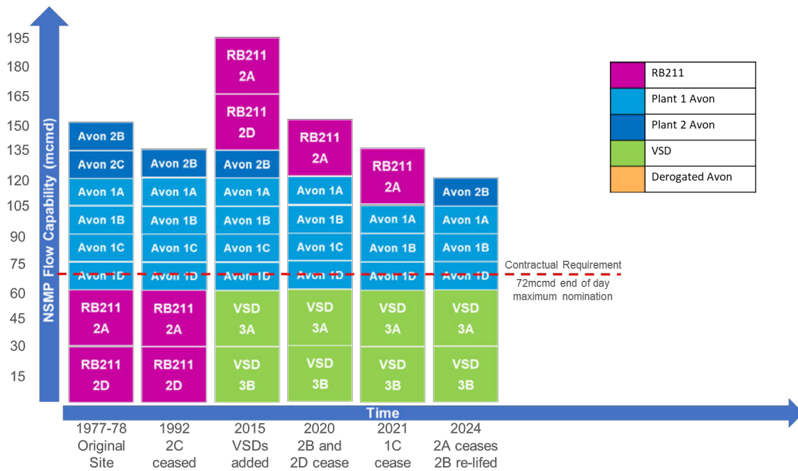
Figure 8 – Site Capacity Changes up to 2030
