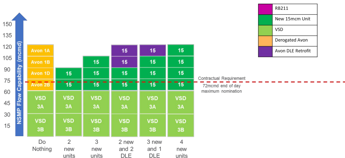
Figure 15 – Site capability under different potential long-term options
