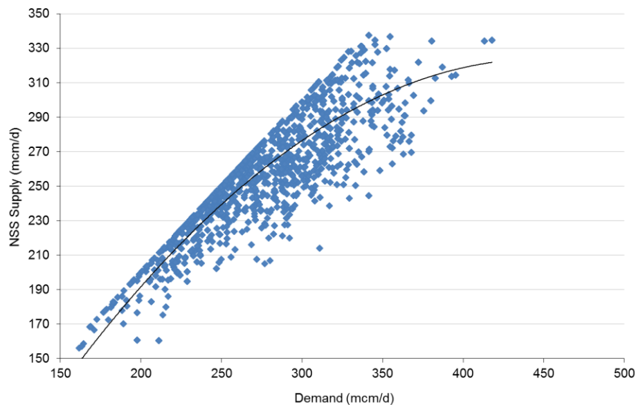
Figure 1 – Non storage supply (NSS) versus demand for the winters 2013/14 to 2017/18
