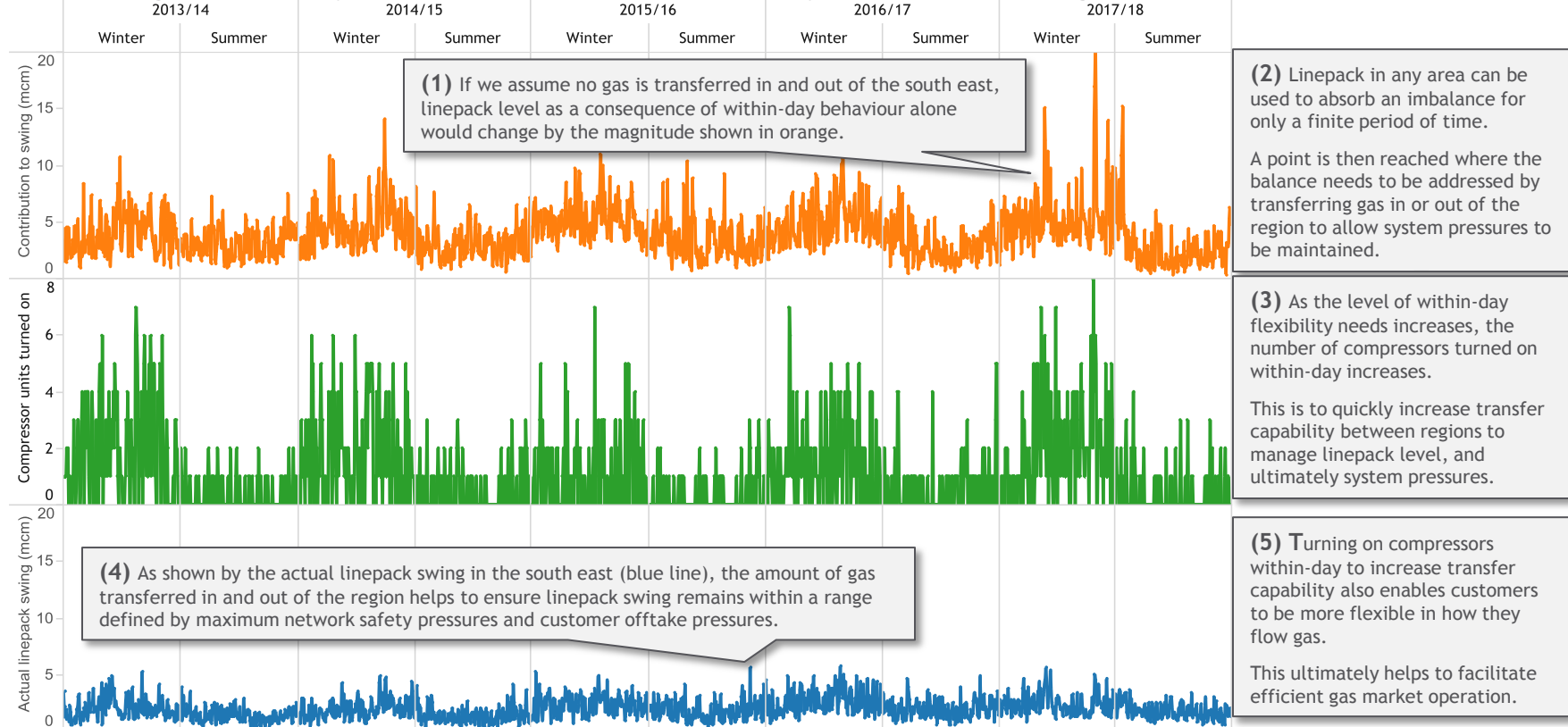
Linepack swing due to within-day behaviour, compressors turned on within-day and actual linepack swing in the south east
