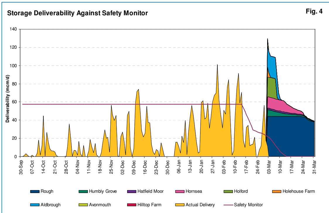
Long Range Storage - Actual Opening Stock Level
