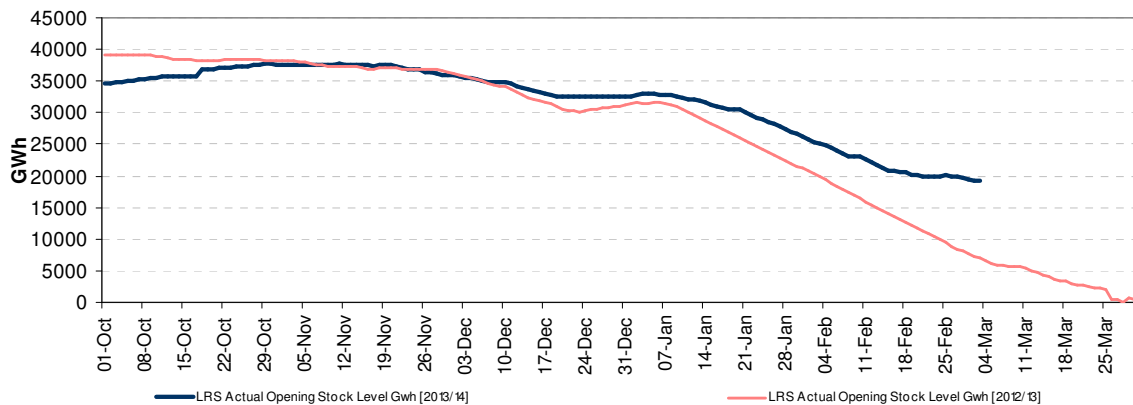
Medium/Short Range Storage - Actual Opening Stock Level
